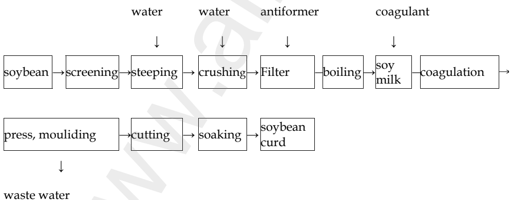
Fig. 4. Manufacturing process of common soybean curd
