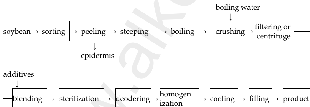
Fig. 5. Processing procedure of soybean milk
