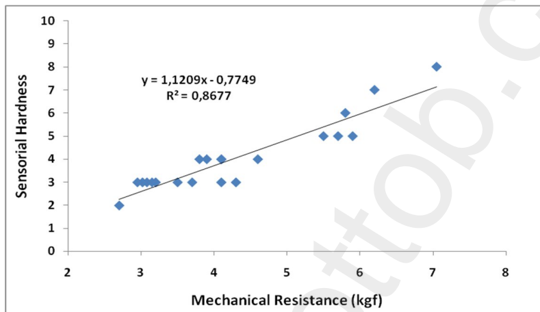
Fig. 4. Relationship between sensorial hardness and mechanical resistance.
