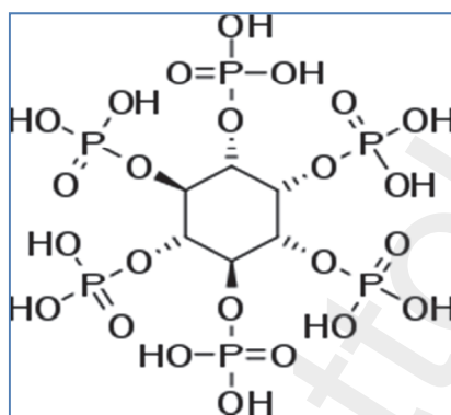
Fig. 2. Molecular structure of Phytic acid
