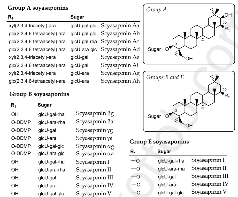
Fig. 2. Chemical structure of the saponins occurring in soy.
