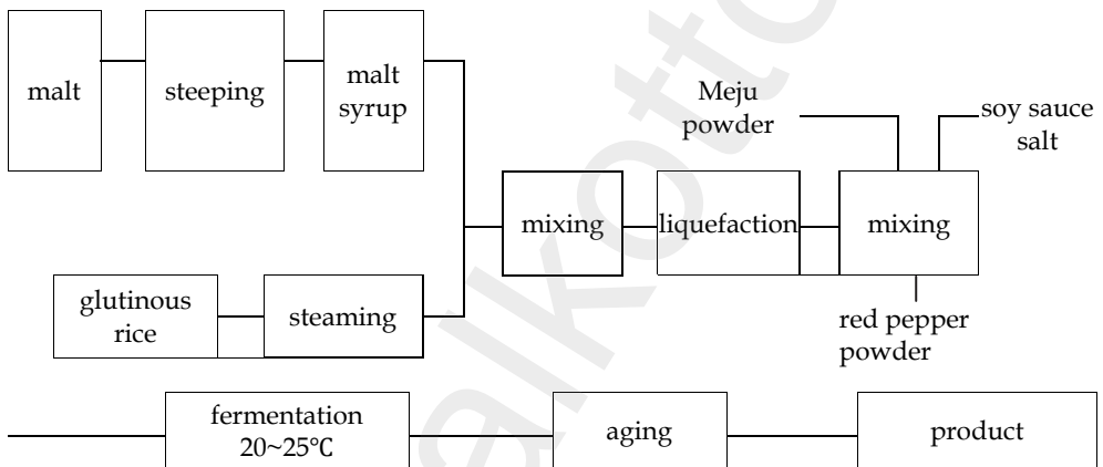
Fig. 9. Process of traditional Gochujang making
