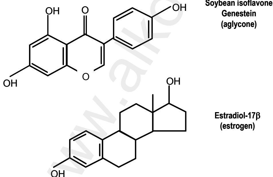
Fig. 1. Molecular structure of soy isoflavone genestein compared to estradiol-17 \beta .
