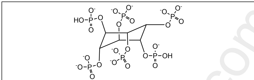
Fig. 3. Chemical structure of myo -inositol-1,2,3,4,5,6-hexakis dihydrogen phosphate.
