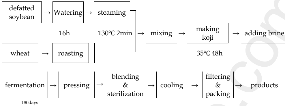
Fig. 7. Common process of Ganjang making
