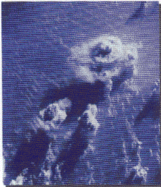
Fig. 18.1 Cumulonimbus clouds seen from space
